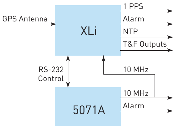
FIG 1 GPS disciplines the cesium 5071A 10MHz master clock within the XLi Time and Frequency System.
