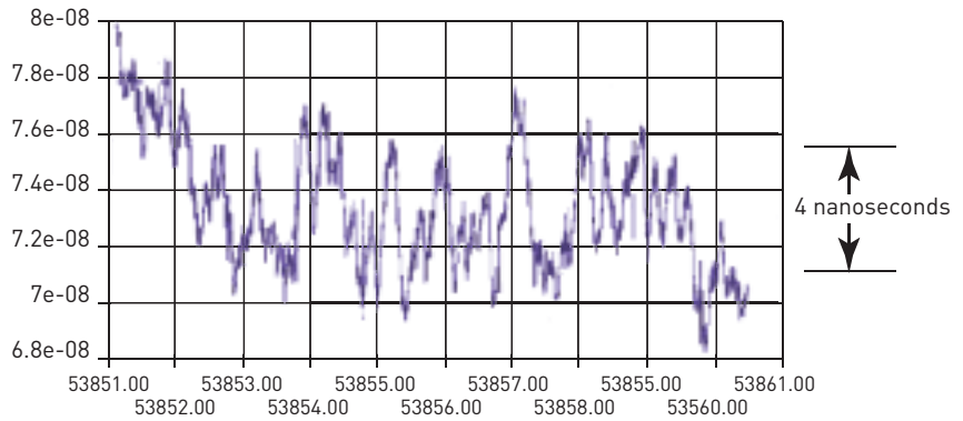
FIG 2 USNO tests of the XLi SAASM 5071 Disciplining Option show root mean square deviations of less than 4ns over 10 days and a cumulative offset of zero.
